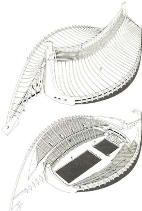
Sports Hall for 1964 Tokyo Olympics
