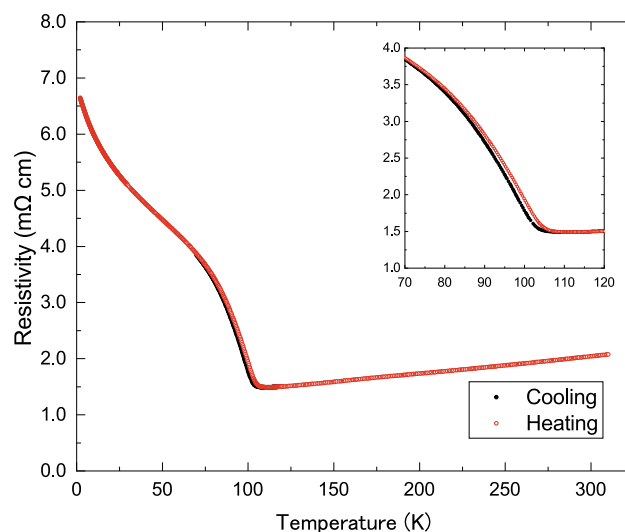
Fig. 7 Electrical resistivity versus temperature curve of sample #4. Closed black circles and open red circles indicate resistivity measured during cooling and heating, respectively. Inset is a magnified view near the transition
