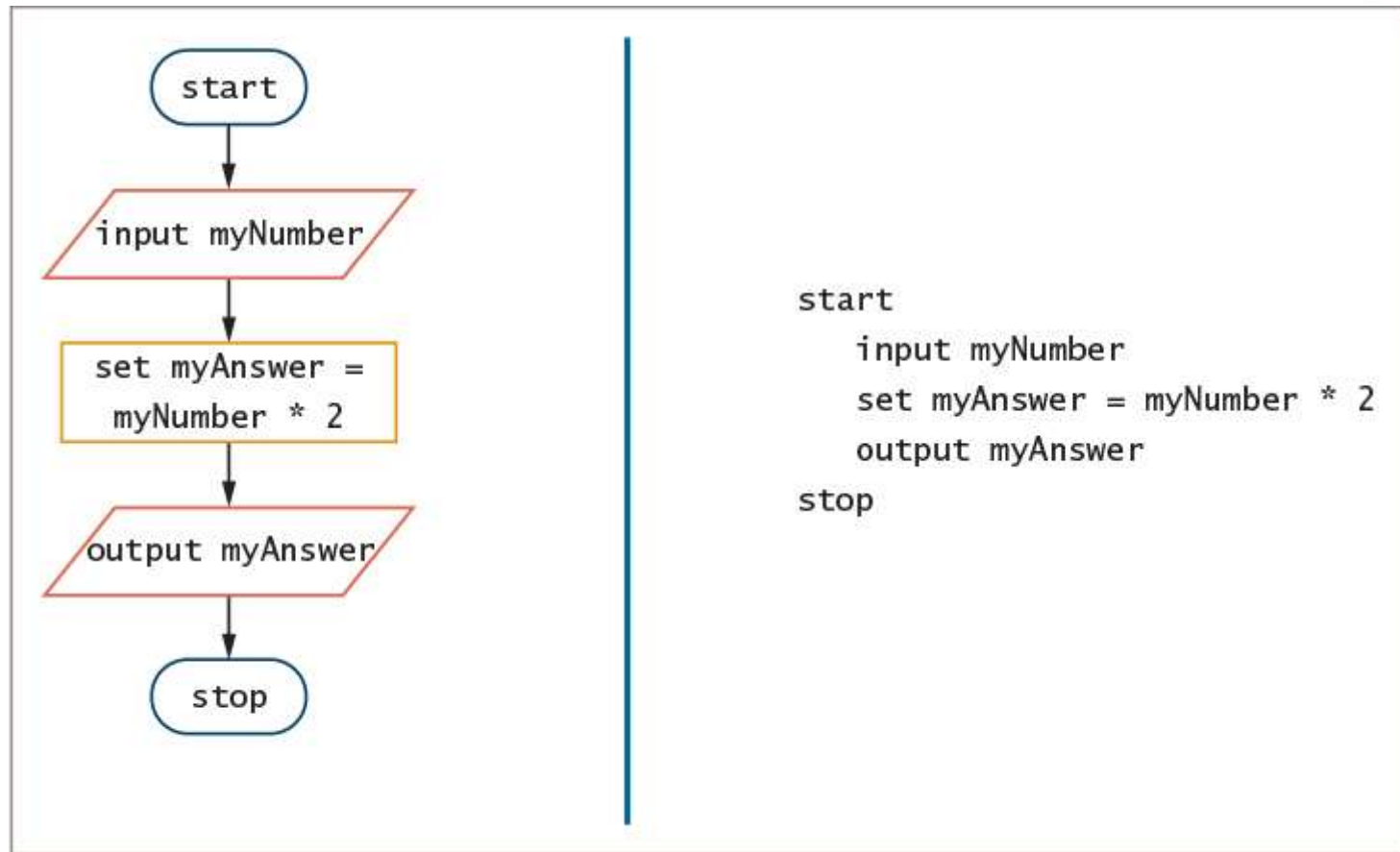
Figure 2-1 Flowchart and pseudocode for the number-doubling program
